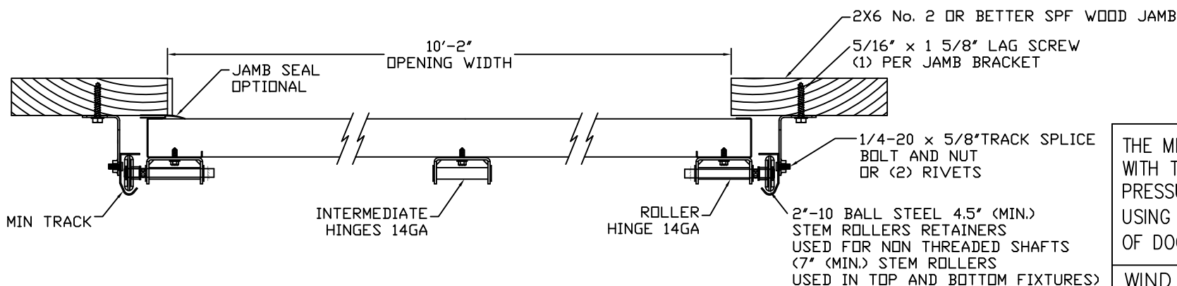
2" BRACKET MOUNT TO WOOD JAMB DETAIL N.T.S.
